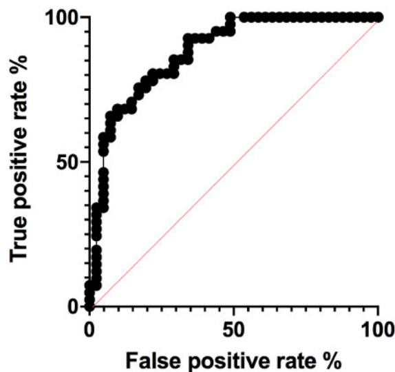
Fig. 3 AUC for REVEL scores
